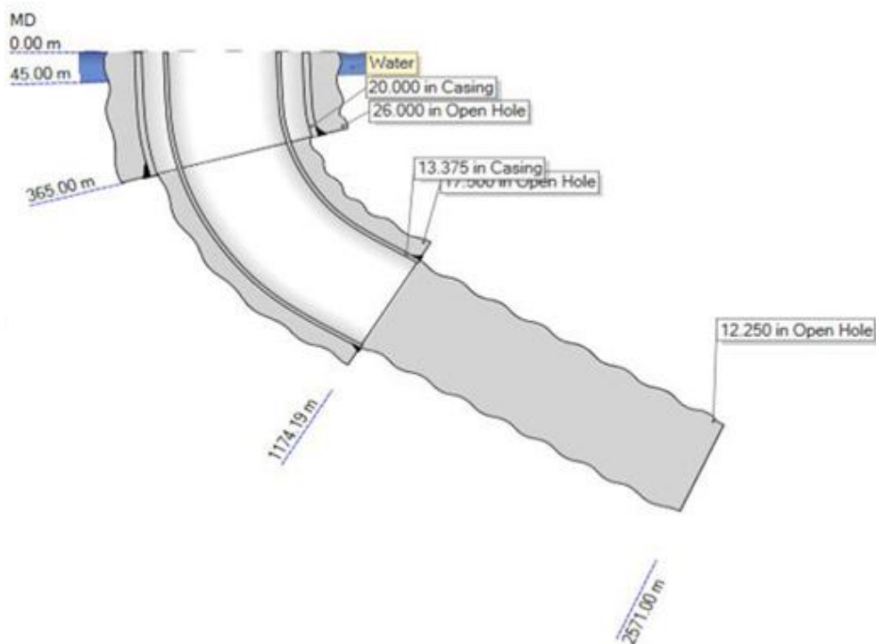
Well Schematic # VSEC-10H
